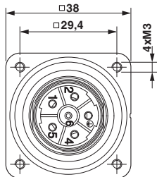
Flange dimensions (Figure shows the 6-pos. version)
